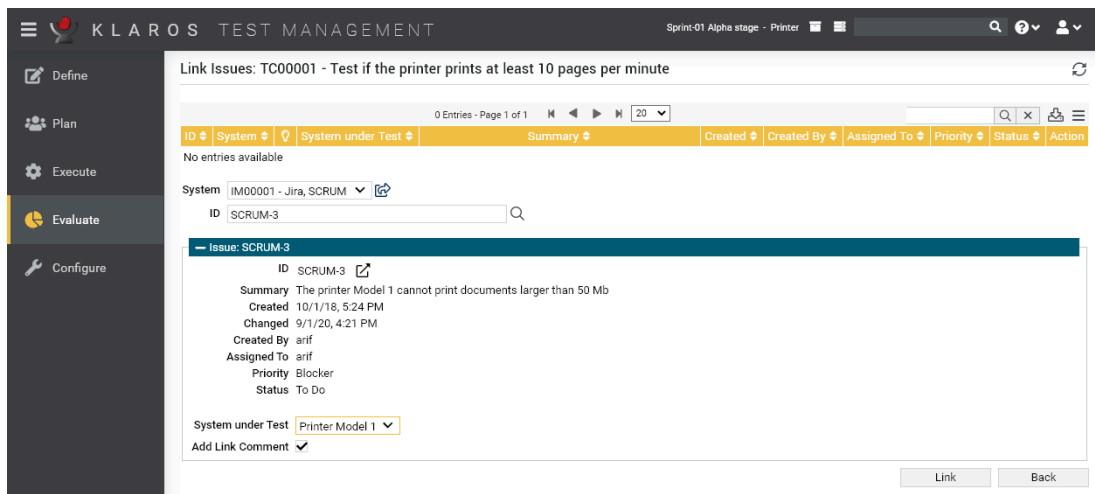
Figure 3.10. Linking Issues
