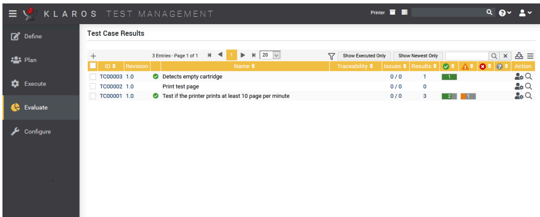
Figure 2.16. The Test Case Results page
